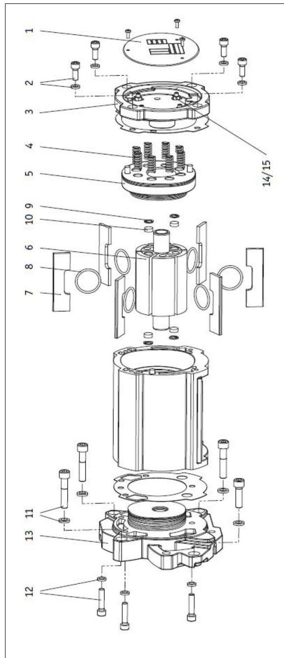
Figure 15: Lifting motor
