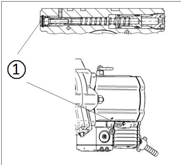
Figure 16: Adjusting overload protection
