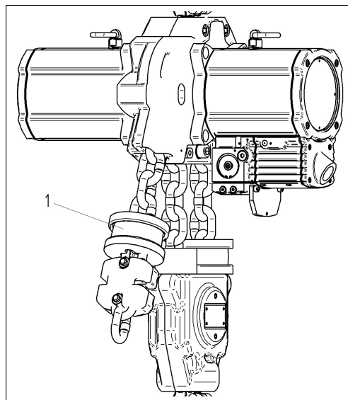
Figure 7: Lowering limiter
