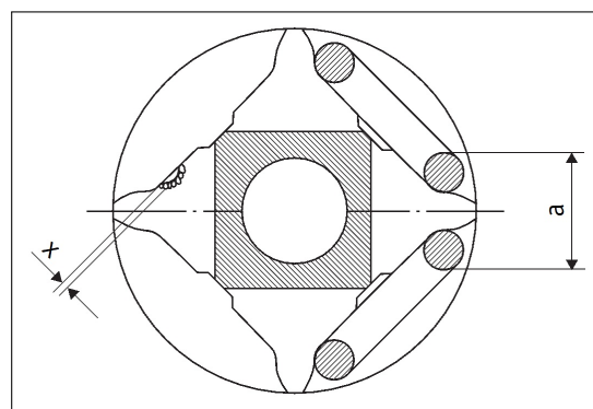
Figure 18: Four-tooth chain sprocket
