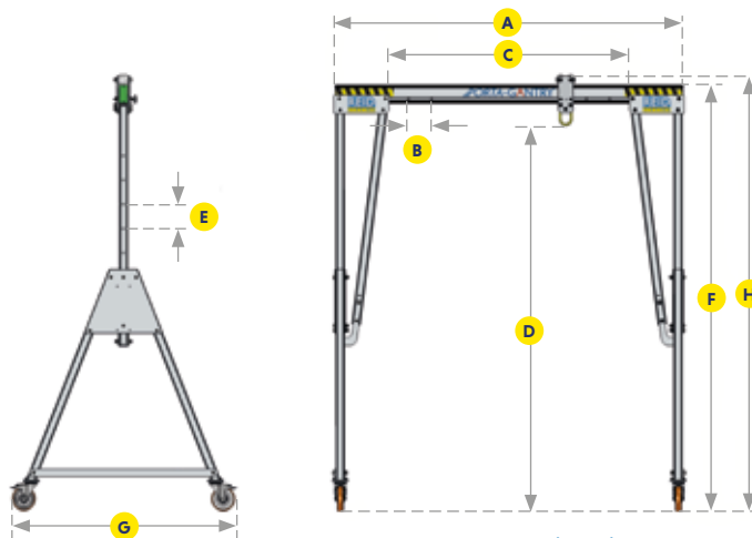
Standard Beam Dimensions
