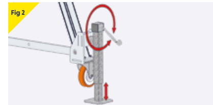
Jacks secured with locking pins and clips
