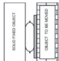
Figure 16 – Separating and Pushing using Air Bags
