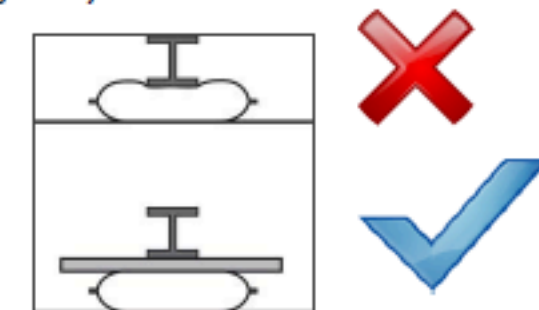
Figure 14 – Small Contact Surface Area
