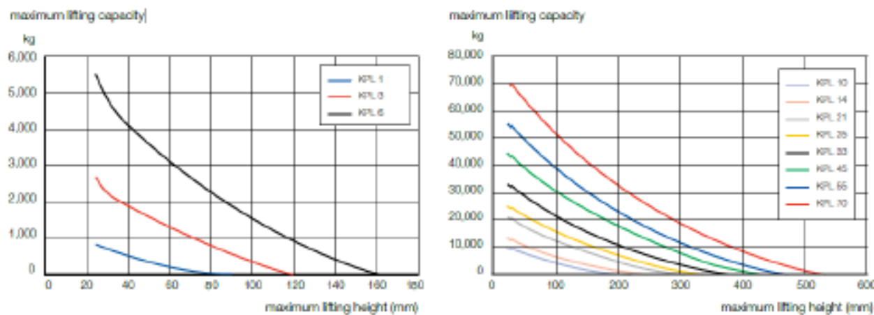
LIFTING CAPACITY VS LIFTING HEIGHT GRAPH
