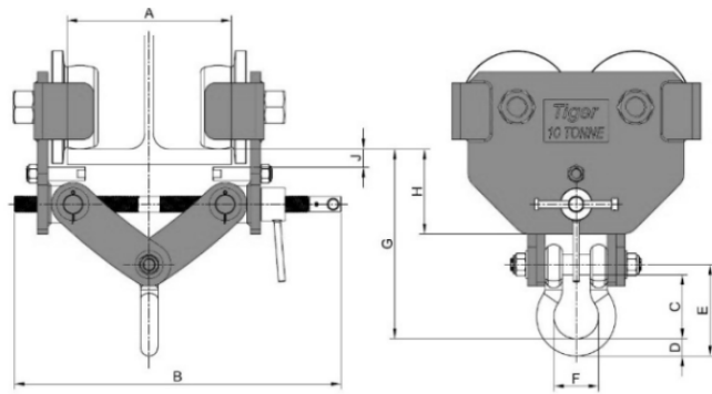
10t Adjustable Plain Trolley (APT)
