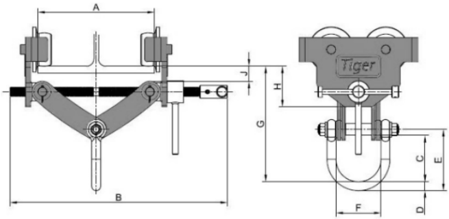
1.0t-6.0t Adjustable Plain Trolley (APT)
