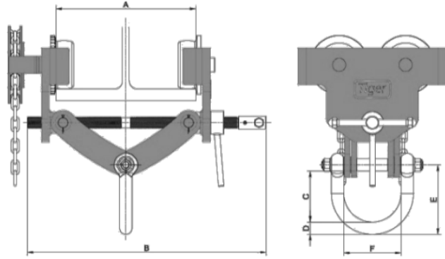
1.0t-6.0t Adjustable Geared Trolley (AGT)
