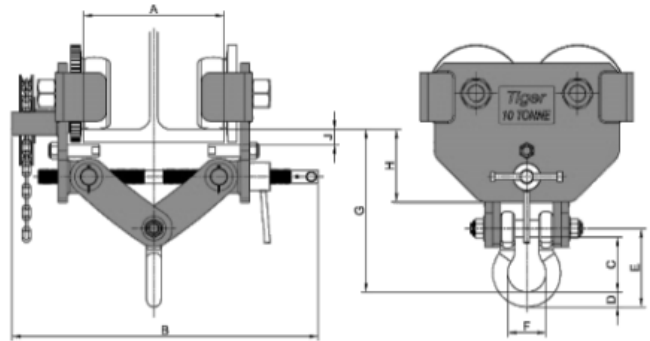
10t Adjustable Geared Trolley (AGT)
