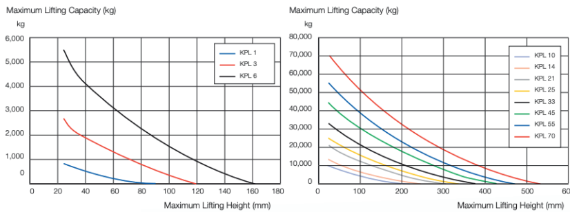
Lifting Capacity vs Lifting Height Graph
